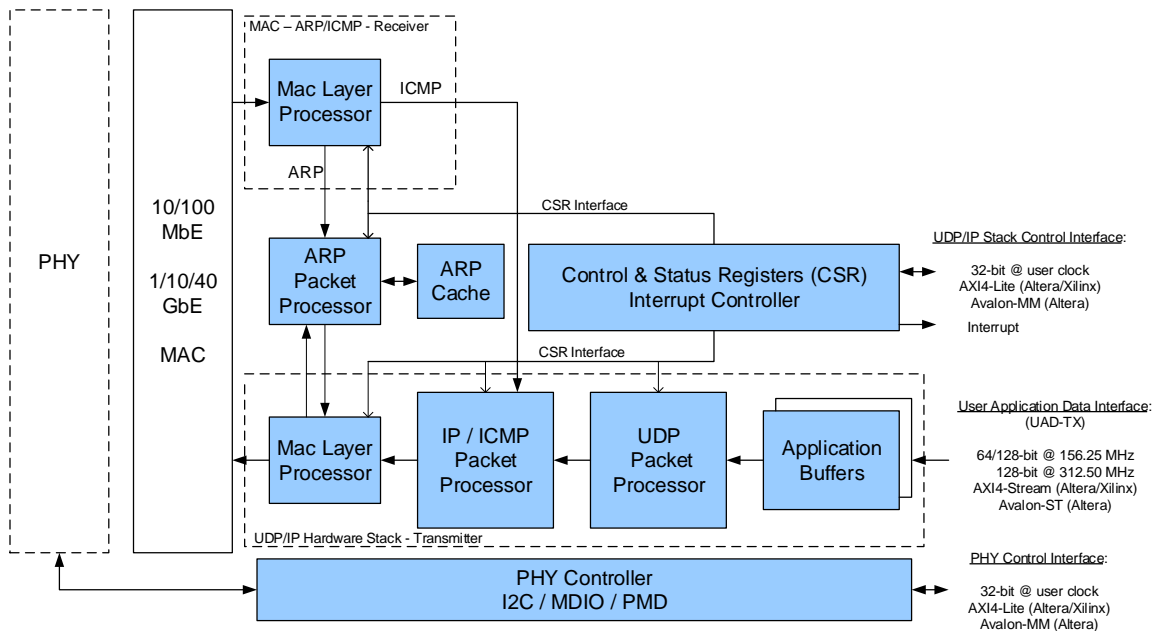
Figure 1: DB-UDP-IP-TX – UDP/IP Hardware Stack for Data Networking Applications – Transmitter Only with ARP and ICMP Support
